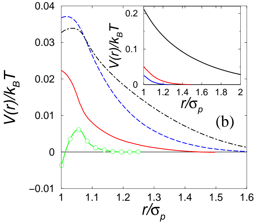
FIG. 10. Total interaction force F(r) (a) and interaction potential V(r) (b) versus dimensionless separation distance r/\sigma_\rho for the DCM at Z = 10 . Solid line- run 7, dashed line- run 8, dot-dashed line- run 9, open circles- run 11. The inset shows low salt concentrations, from top to bottom: runs 1, 4, 5.
