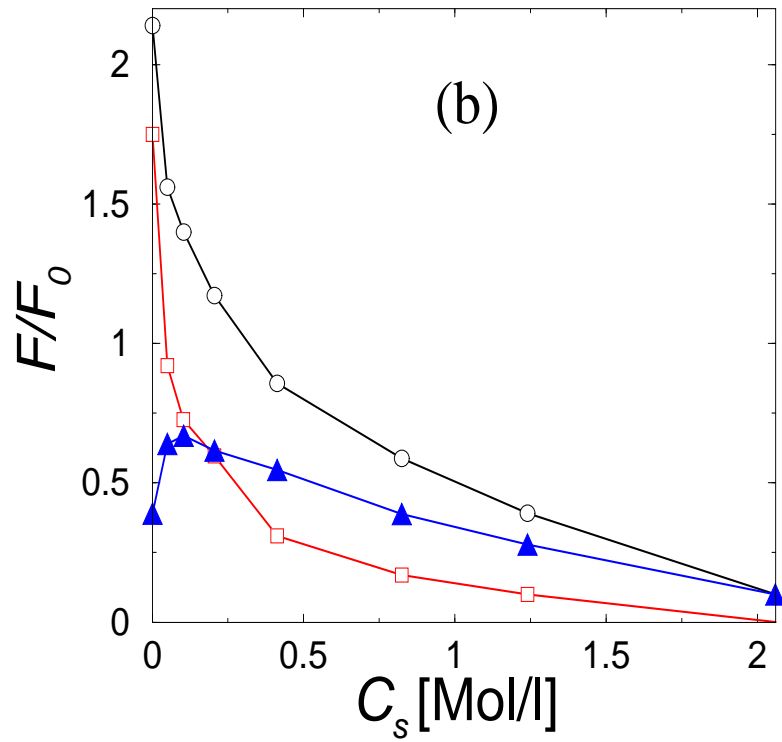
FIG. 8. The total interaction force F (circles) and its electrostatic, F^{(2)} (squares) and entropic F^{(3)} (triangles) components versus salt concentration. The separation distance is fixed at (a) r/\sigma_p = 1 and (b) r/\sigma_p = 1.1 . The simulations are for the SCM with Z = 10 , and show that at high salt concentrations, the entropic force dominates.
