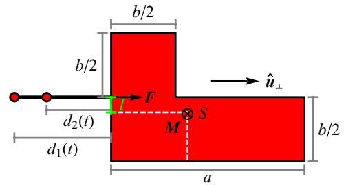
Figure 1. Schematic of a force-free and torque-free L-shaped Golestanian-like microswimmer of size a and orientation \hat{\mathbf{u}}_{\perp} . To put the microswimmer in motion, the distances d_1(t) and d_2(t) of the two small spheres from the L-shaped particle, which vary as a non-reciprocal function of time. The effective lever arm l relates the effective force \mathbf{F} to the effective torque \mathbf{M} = \|\mathbf{M}\| on the centre of mass S .
