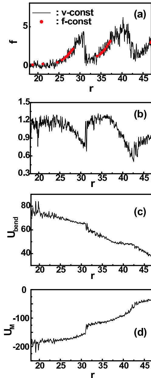
FIG. 7: Unwrapping process by stretching an end monomer by a constant speed for the chain stiffness parameter \kappa = 10 . (a) Force-extension relation. The result from the force constant ensemble is also plotted by circles for comparison. (b) Tilting angle-extension relation. (c) Bending energy-extension relation. (d) Adsorption energy-extension relation.
