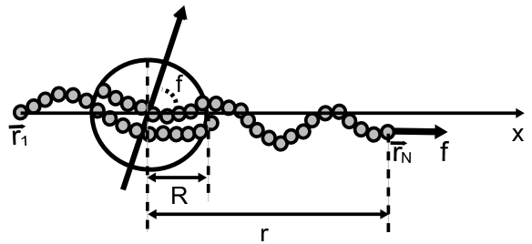
FIG. 1: Schematic sketch of the complex under external stretching. The first end monomer is fixed at \mathbf{r}_1 , the protein sphere with radius R is fixed at the origin and the other end monomer is pulled by the force f along the x axis. The chain extension r , and the tilt angle \phi , which can be defined for the ordered complex, are also shown.
