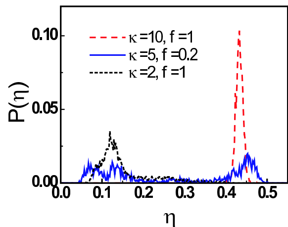
FIG. 3: Probability distribution of the order parameter \eta for complexes made from chains with different stiffnesses \kappa = 2, 5 and 10 under a stretching force f .
