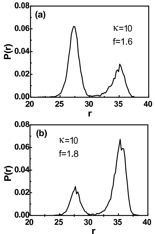
FIG. 6: Probability distribution of the chain extension r (a) below ( f=1.6 ) and (b) above ( f=1.8 ) the critical stretching force to induce the unwrapping transition from w = 2 to w = 1 for the chain stiffness of \kappa = 10 .
