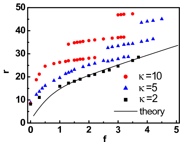
FIG. 2: (Dot) Force-extension relation of the sphere-chain complex obtained by computer simulations for different chain stiffnesses \kappa = 2, 5 and 10 . In case of a bimodal distribution of r , we plot both peak positions. (Line) Theoretical force-extension relation of the disordered sphere-chain complex. The parameters are estimated from the corresponding system in the simulation with \kappa = 2 : a_1 = -7 , a_2 = 0.12 , L_0 = 44 , \lambda_p = 1.5 .
