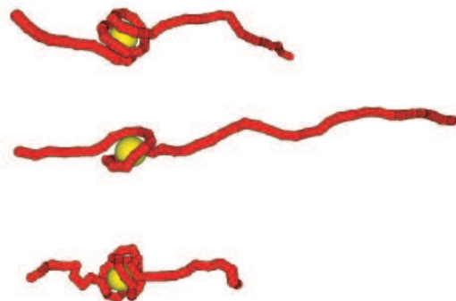
FIG. 4: Typical simulation snapshots of the sphere-chain complex. Top: an ordered wrapping with wrapping number w = 2 for \kappa = 10 , f = 1 . Middle: an ordered wrapping with w = 1 for \kappa = 10 , f = 2.5 . Bottom: a disordered state for \kappa = 2 , f = 1 .
